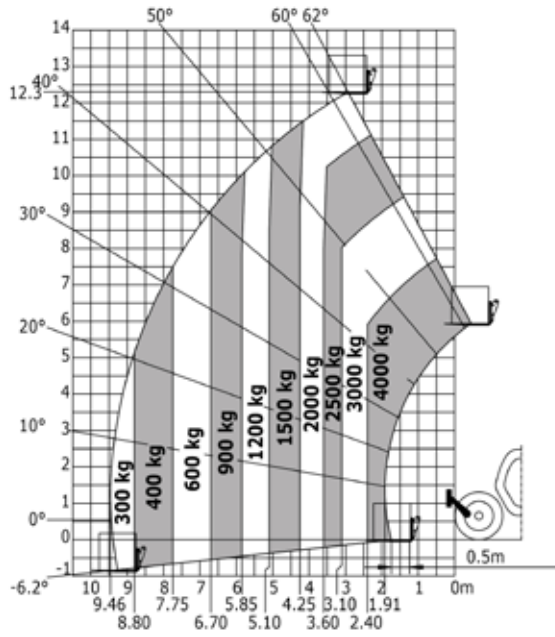
Machine on tyres with forks - with levelling
