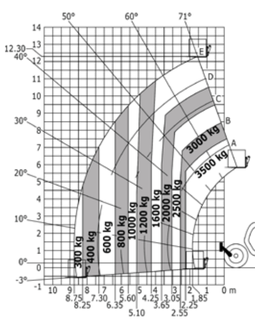
Machine on tyres with forks - with levelling
