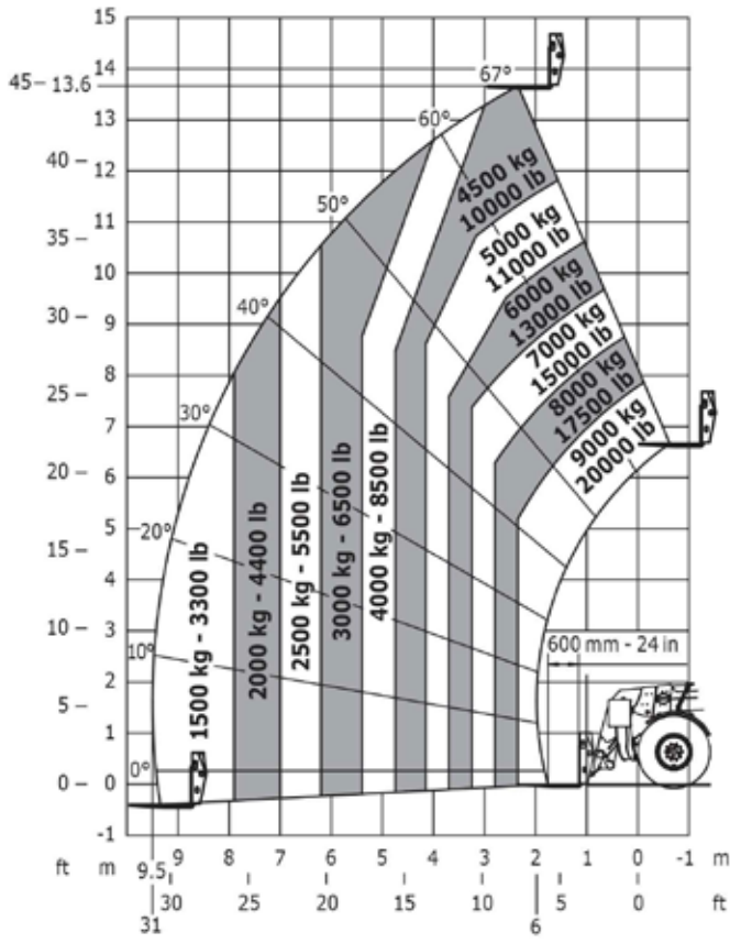
Machine on tyres with forks - CoG 600 mm
