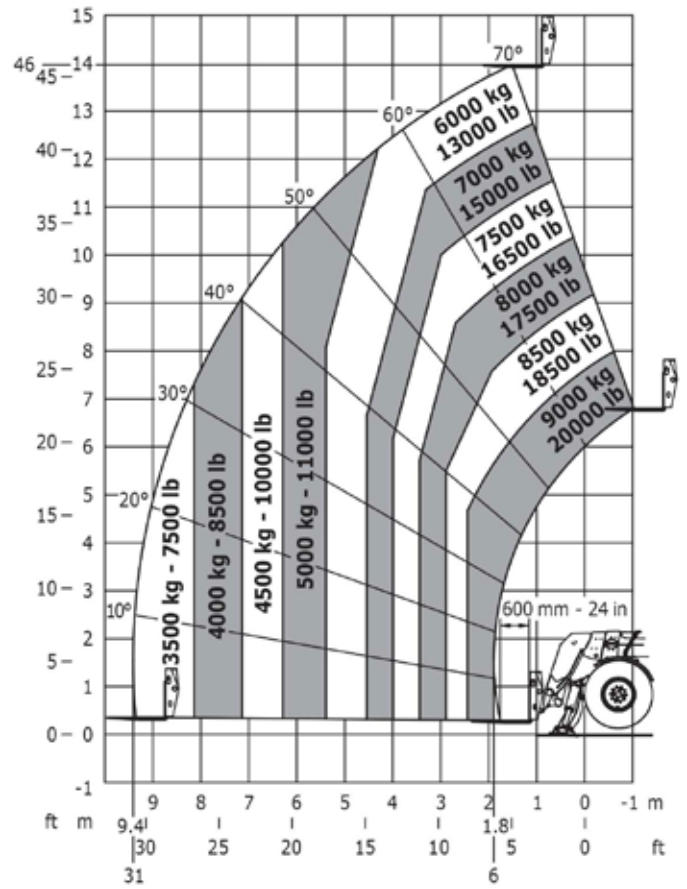
Rotation on lowered stabilisers with forks - CoG 600 mm
